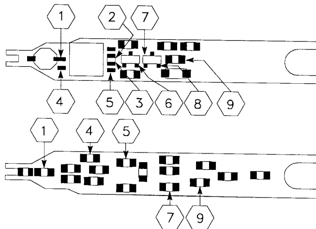
Figure 9-1. Probe body circuit board for instrument numbers 8848 and up.
