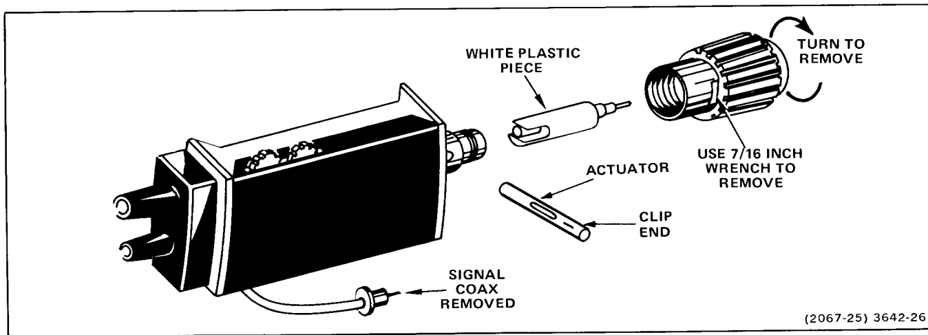
Figure 5-7. INT-EXT switch removal.
