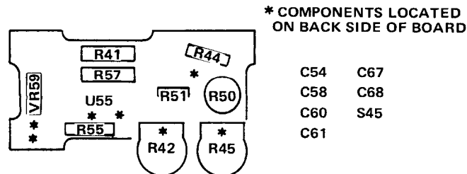
Figure 9-2. Probe control body circuit board.
