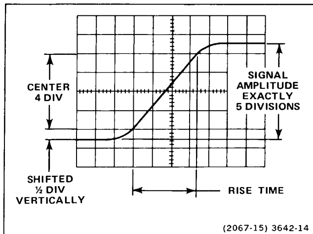
Figure 4-3. Rise time.
