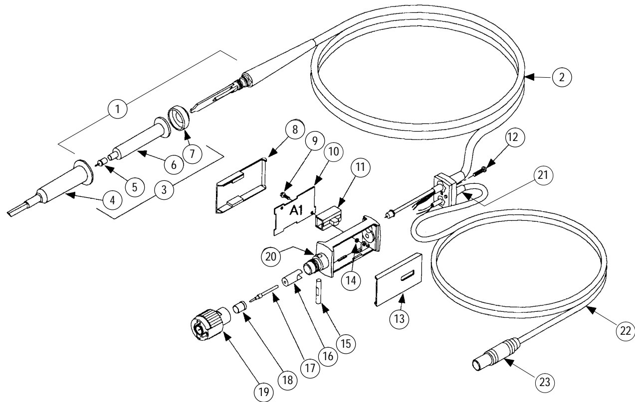
Figure 8-1: Exploded view
